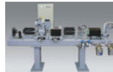
Villares Metals, Brazil: Test Section for wire with CIRCOGRAPH Ro 20 + DEFECTOMAT channel M 40 + EMAG M
